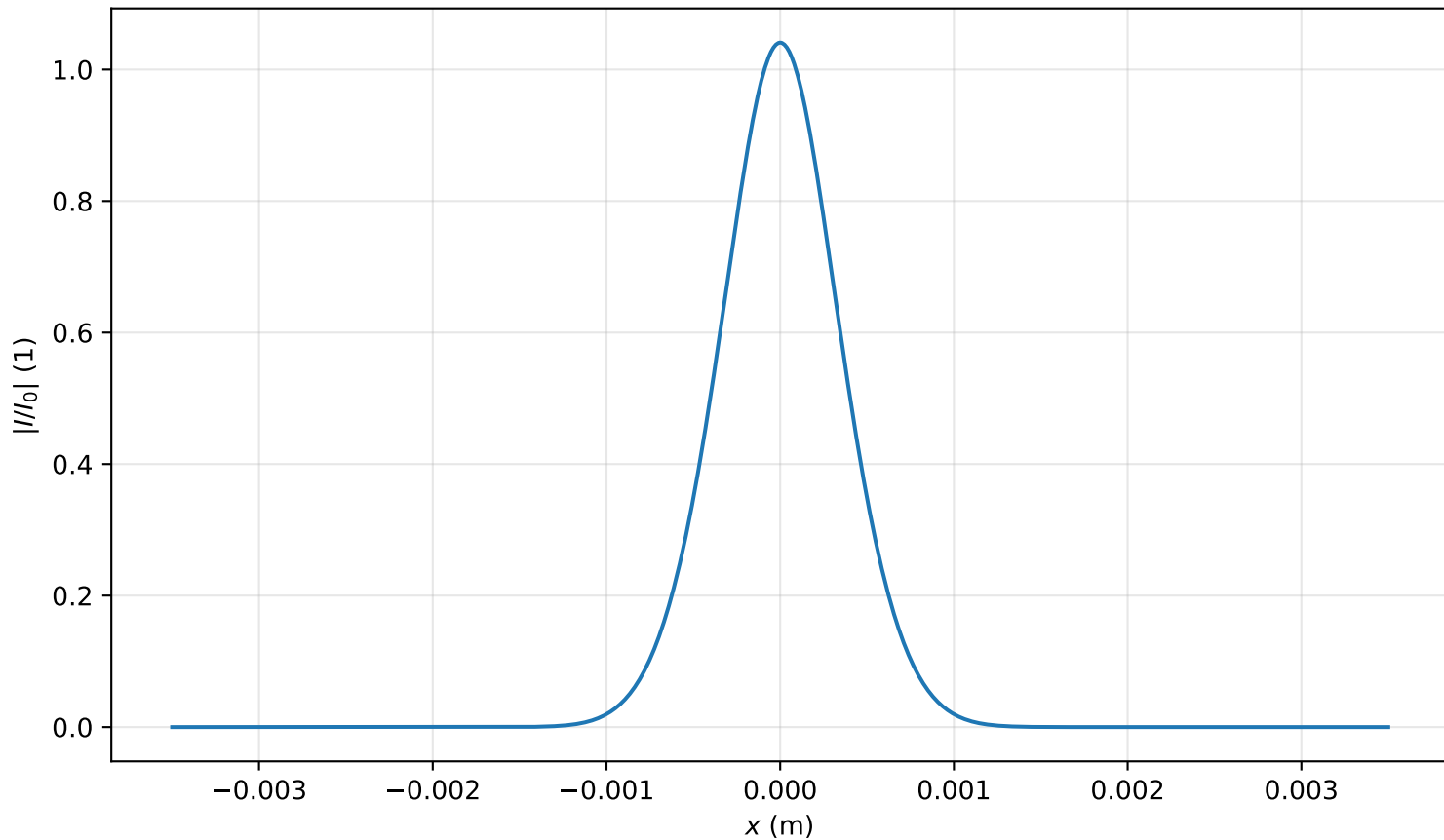
Intensity profile I(x, y = 0, z = 0.478m)/I_0 , P_{in}=0.5P_{cr} , artificial time
